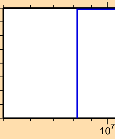
\sigma vs. E for ^{13}\text{N}(\text{mt117})
