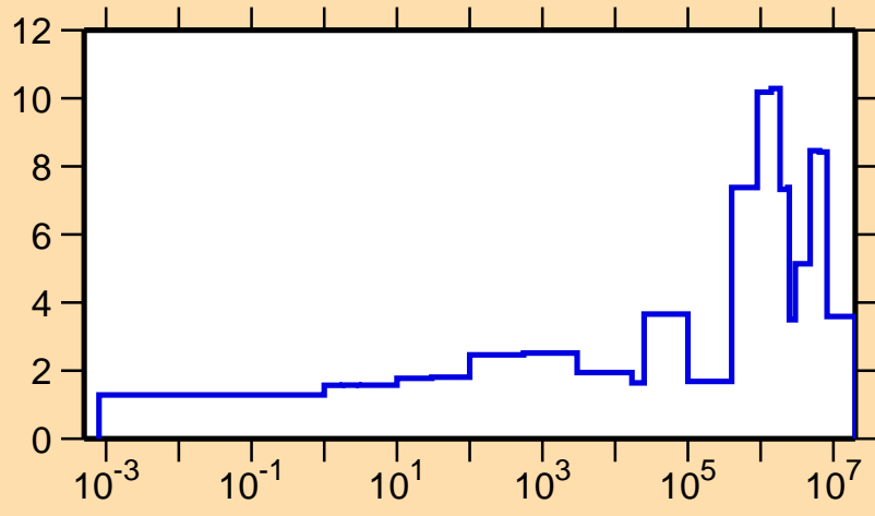
\Delta\sigma/\sigma vs. E for ^{13}\text{N}(n,el.)
