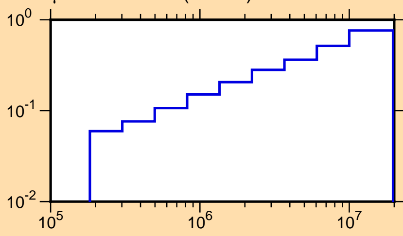
\mu vs. E for ^{16}\text{N}(\text{mt251})
