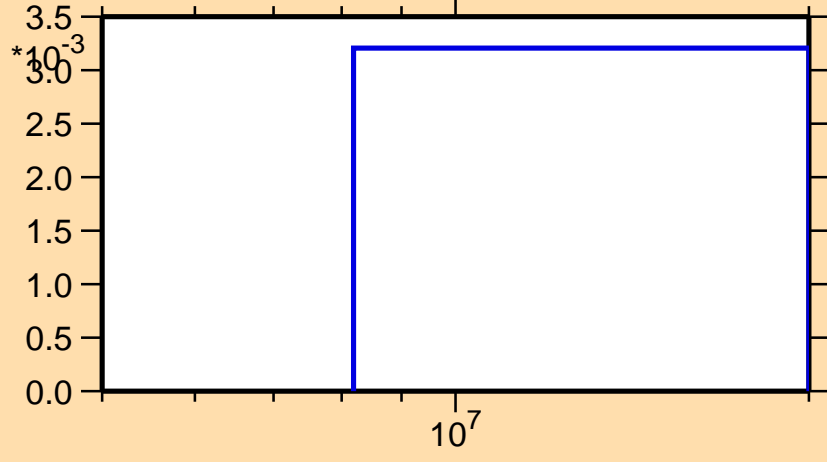
\sigma vs. E for ^{16}\text{N}(n,\text{nd})
