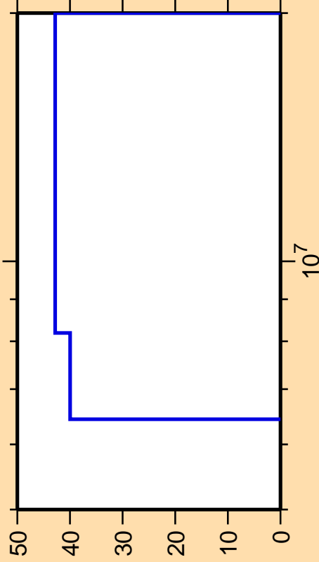
\Delta\sigma/\sigma vs. E for ^{16}\text{N}(n,p)
