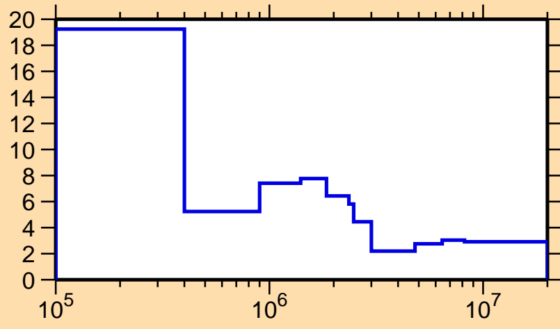
\Delta\sigma/\sigma vs. E for ^{16}\text{N}(n,\text{tot.})
