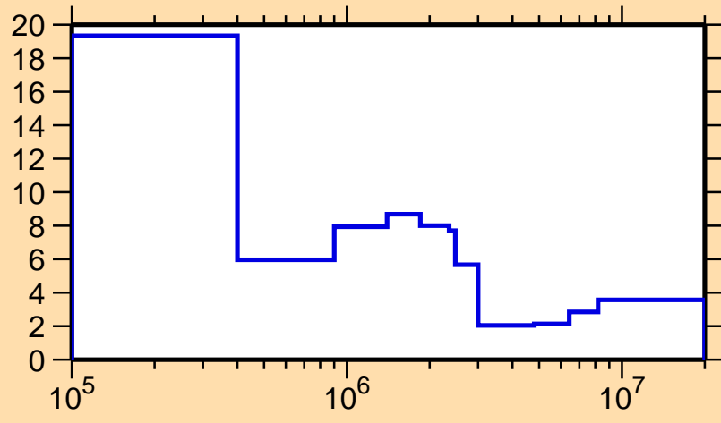
\Delta\sigma/\sigma vs. E for ^{16}\text{N}(n,\text{el.})
