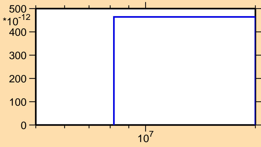
\sigma vs. E for ^{17}\text{N}(n,2np)
