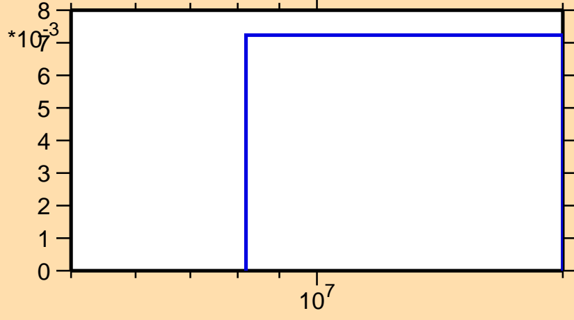
\sigma vs. E for ^{17}\text{N}(n,t)
