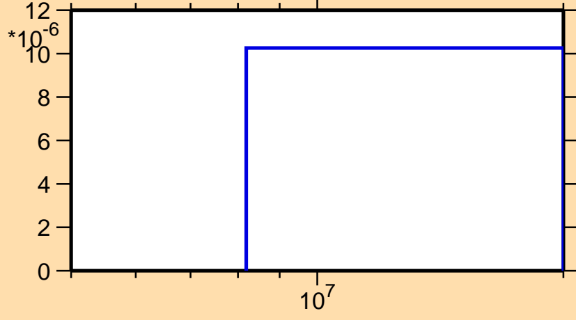
\sigma vs. E for ^{17}\text{N}(n,nd)
