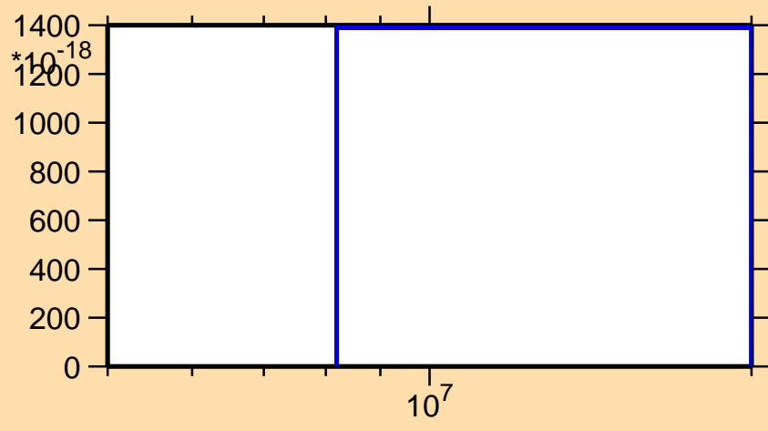
\sigma vs. E for ^{17}\text{N} (mt 42)
