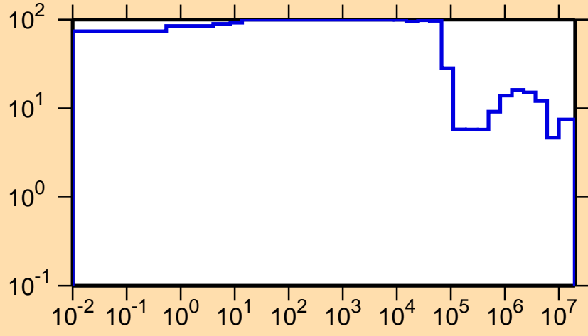
\Delta\sigma/\sigma vs. E for ^{21}\text{Na}(n,el.)
