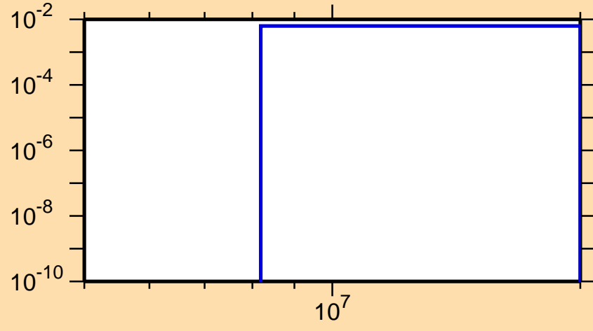
\sigma vs. E for ^{21}\text{Na} (mt 45)
