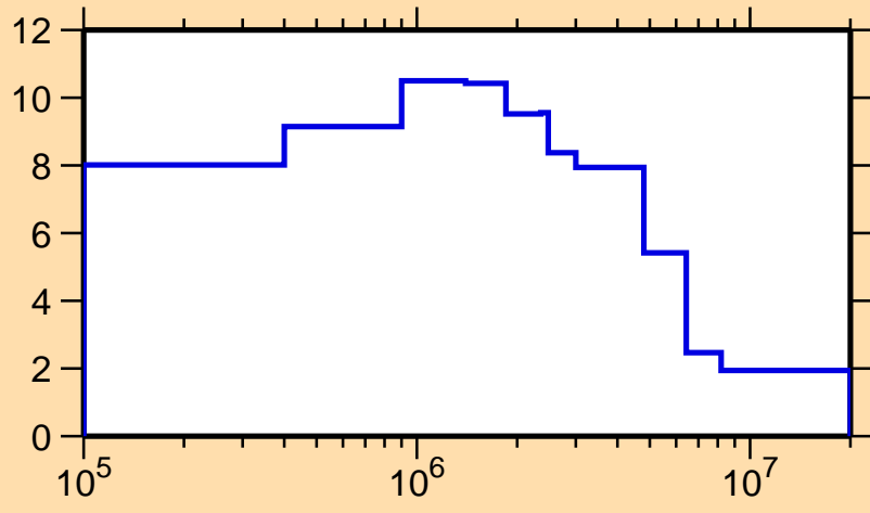
\Delta\sigma/\sigma vs. E for ^{21}\text{Na}(n,\text{tot.})
