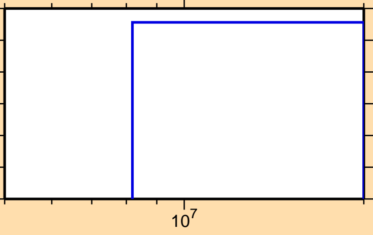
\sigma vs. E for ^{21}\text{Na}(n,2n)
