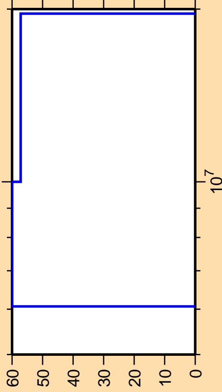
\Delta\sigma/\sigma vs. E for ^{22}\text{Na}(n,p\alpha)
