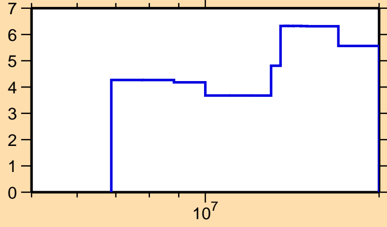
\Delta\sigma/\sigma vs. E for ^{23}\text{Na}(n,n\text{onel.})
