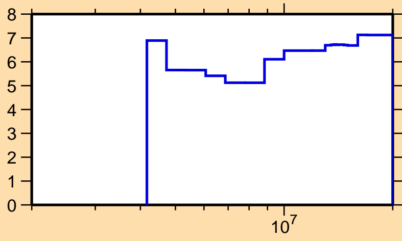
\Delta\sigma/\sigma vs. E for ^{24}\text{Na}(n,n\text{onel.})
