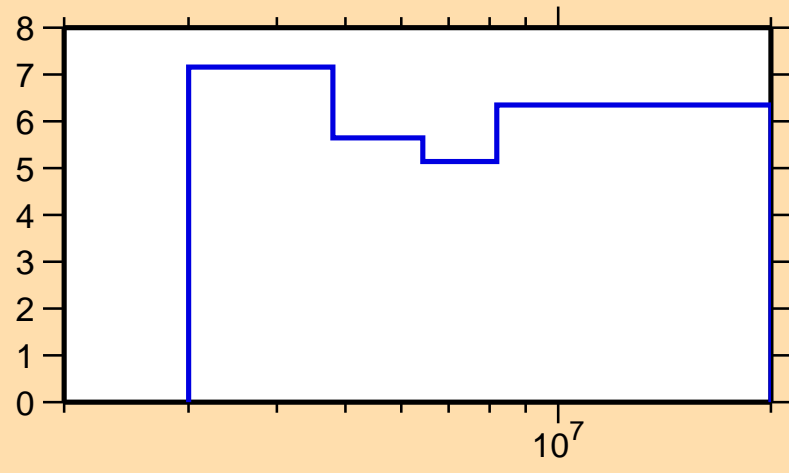
\Delta\sigma/\sigma vs. E for ^{24}\text{Na}(n,n\text{nonel.})
