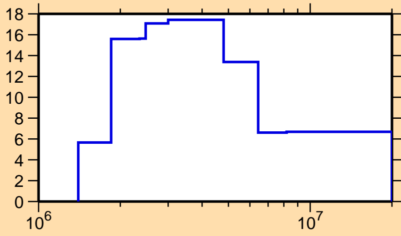
\Delta\sigma/\sigma vs. E for ^{24}\text{Na}(n,el.)
