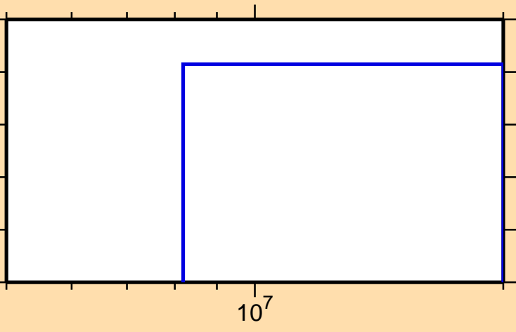
\sigma vs. E for ^{24}\text{Na}(n,2np)
