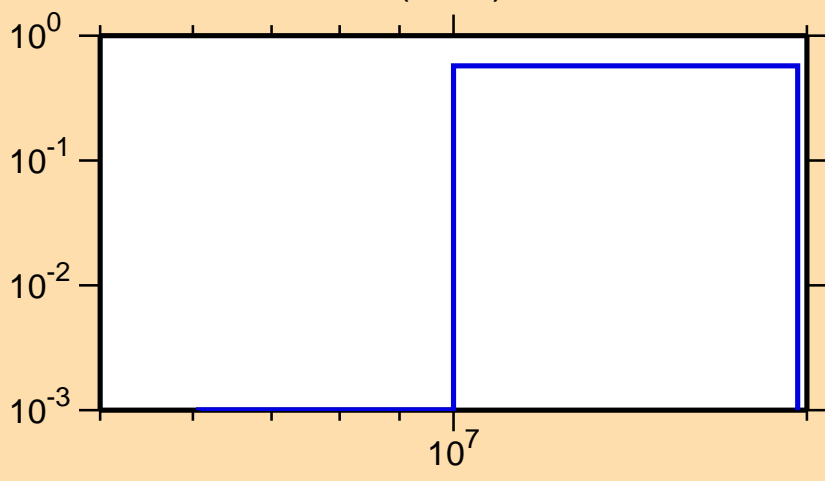
\sigma vs. E for ^{25}\text{Na}(n,2n)
