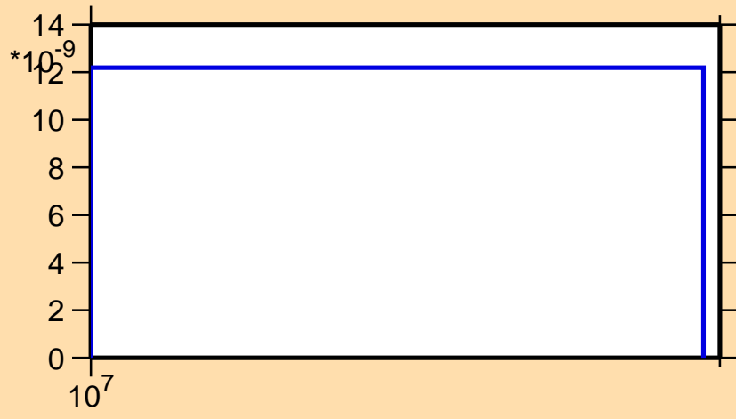
\sigma vs. E for ^{25}\text{Na}(n,nd)
