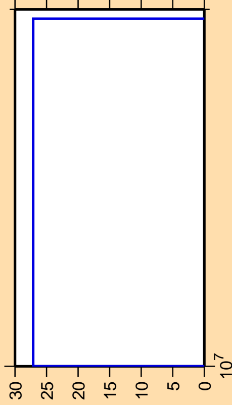
\Delta\sigma/\sigma vs. E for ^{25}\text{Na}(n,nd)
