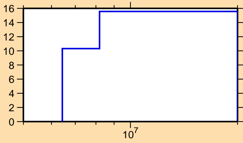
\Delta\sigma/\sigma vs. E for ^{25}\text{Na}(n,ncont.)
