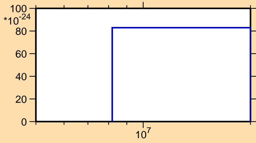
\sigma vs. E for ^{25}\text{Na}(n,p\alpha)
