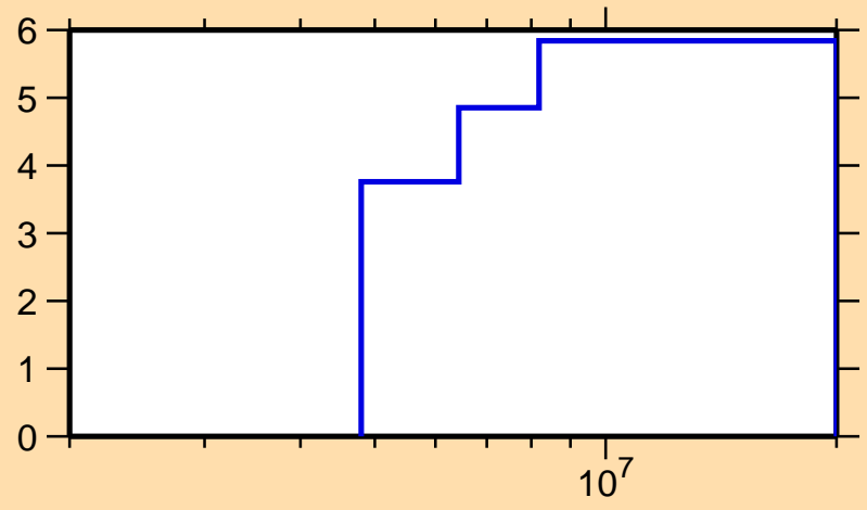
\Delta\sigma/\sigma vs. E for ^{25}\text{Na}(n,n\text{nonel.})
