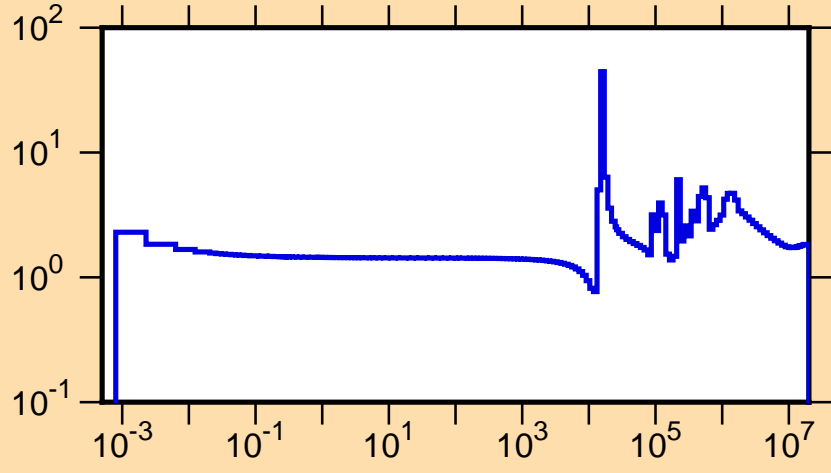
\sigma vs. E for ^{26}\text{Na}(n,\text{tot.})
