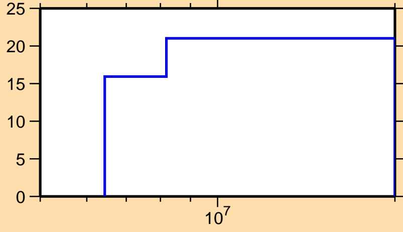
\Delta\sigma/\sigma vs. E for ^{26}\text{Na}(n,ncont.)
