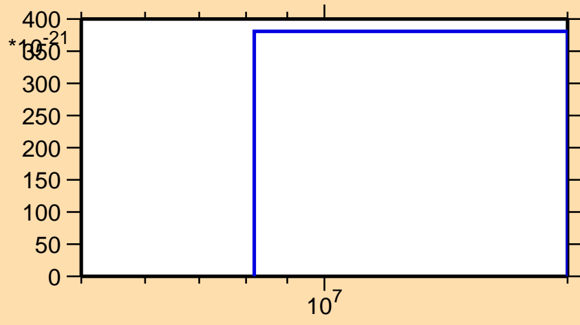
\sigma vs. E for ^{26}\text{Na}(n,p\alpha)
