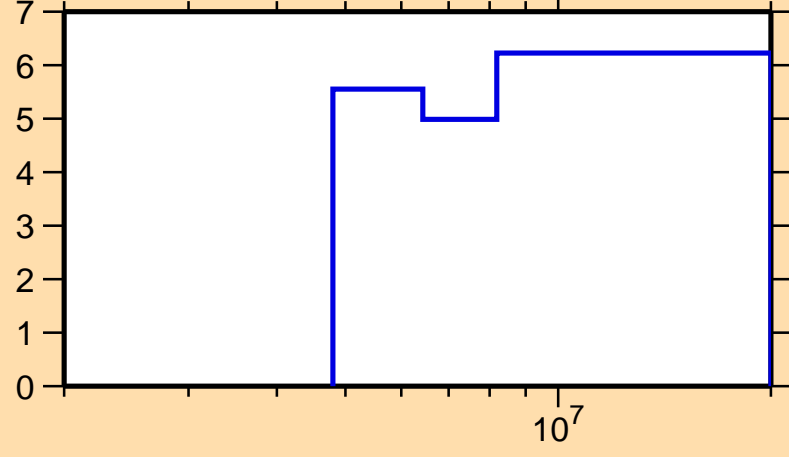
\Delta\sigma/\sigma vs. E for ^{26}\text{Na}(n,\text{nonel.})
