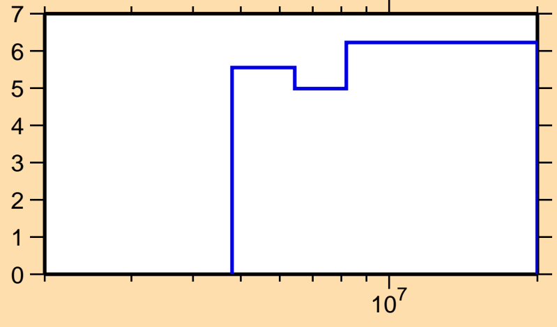
\Delta\sigma/\sigma vs. E for ^{26}\text{Na}(n,n\text{nonel.})
