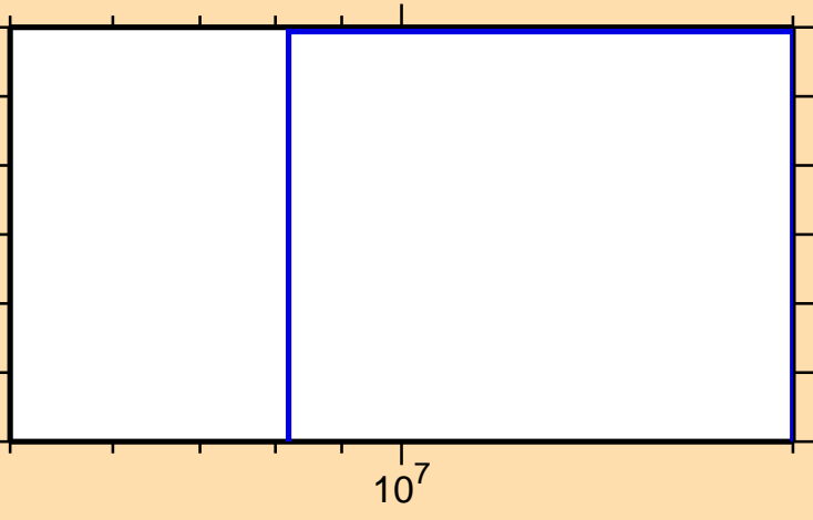
\sigma vs. E for ^{26}\text{Na}(n,nt)
