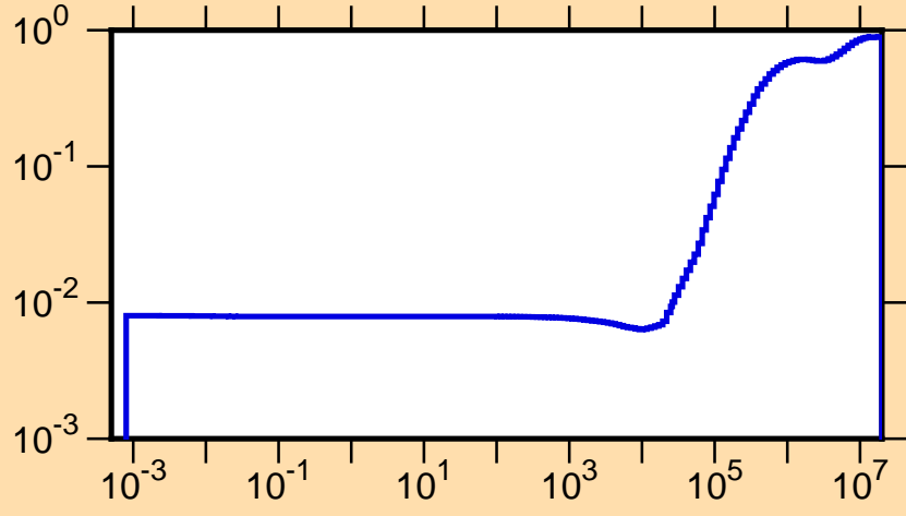
\mu vs. E for ^{84}\text{Nb}(\text{mt251})
