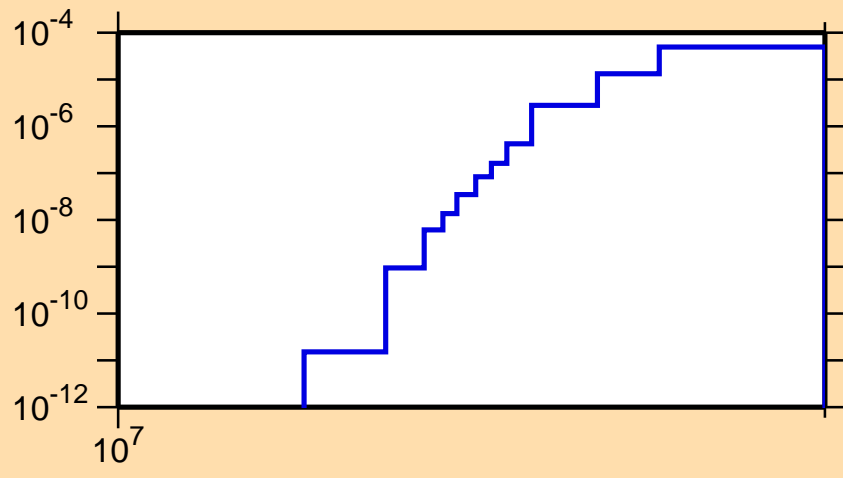
\sigma vs. E for ^{84}\text{Nb}(n,\text{nd})
