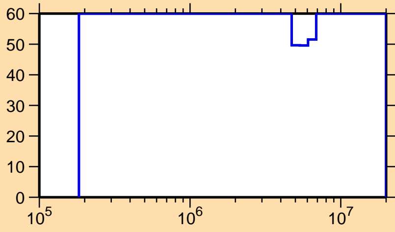
\Delta\sigma/\sigma vs. E for ^{84}\text{Nb}(n,n\text{cont.})
