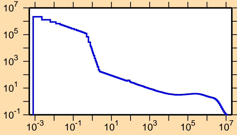
\sigma vs. E for ^{84}\text{Nb}(n,p)
