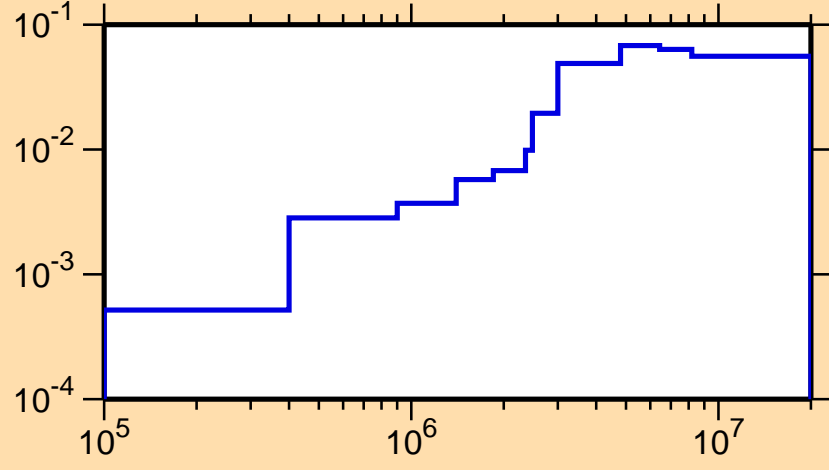
\sigma vs. E for ^{84}\text{Nb}(n,n\text{cont.})
