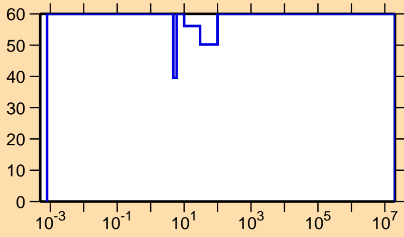
\Delta\sigma/\sigma vs. E for ^{84}\text{Nb}(n,\gamma)
