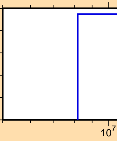
\sigma vs. E for ^{84}\text{Nb}(\text{mt } 45)
