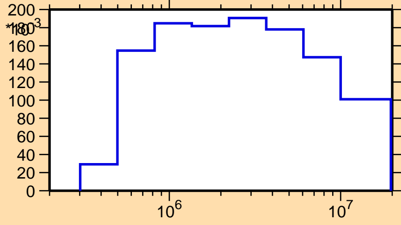
\sigma vs. E for ^{85}\text{Nb}(n,\text{inel.})
