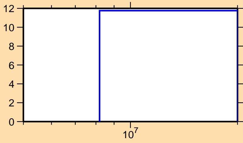
\Delta\sigma/\sigma vs. E for ^{85}\text{Nb}(n,\text{tot.})
