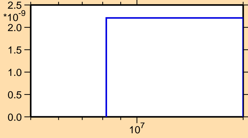
\sigma vs. E for ^{85}\text{Nb}(n,\text{pt})
