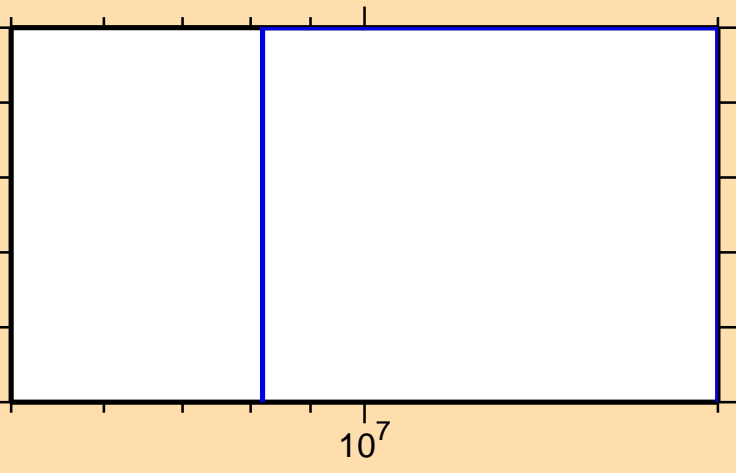
\sigma vs. E for ^{85}\text{Nb}(n,2n)
