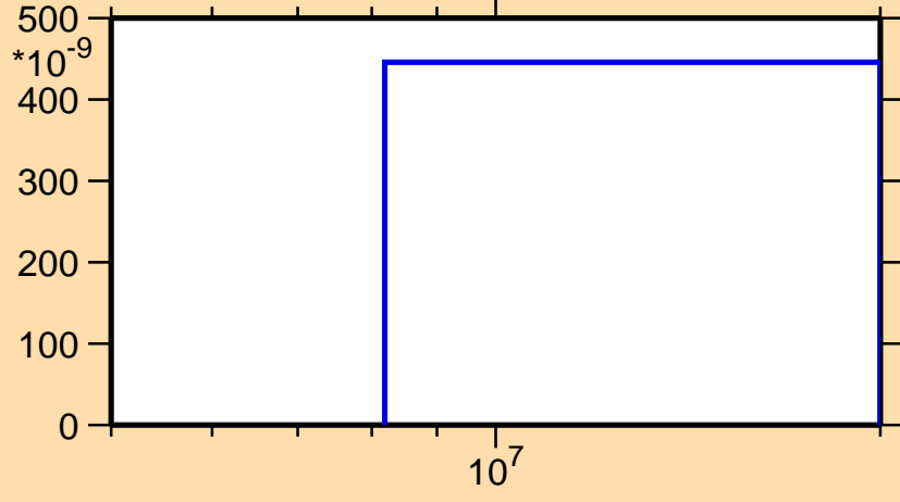
\sigma vs. E for ^{85}\text{Nb} (mt 45)
