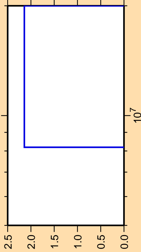
\Delta\sigma/\sigma vs. E for ^{85}\text{Nb} (mt 34)
