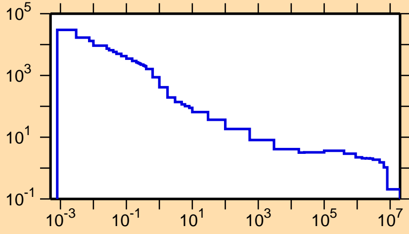
\sigma vs. E for ^{85}\text{Nb}(n,p)
