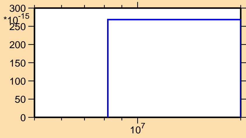
\sigma vs. E for ^{85}\text{Nb} (mt 34)
