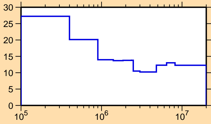
\Delta\sigma/\sigma vs. E for ^{85}\text{Nb}(n,n\text{nonel.})
