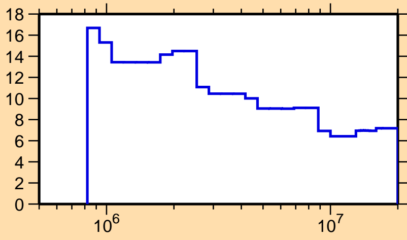
\Delta\sigma/\sigma vs. E for ^{86}\text{Nb}(n,n\text{onel.})
