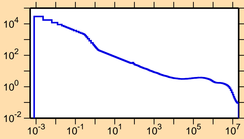
\sigma vs. E for ^{86}\text{Nb}(n,p)
