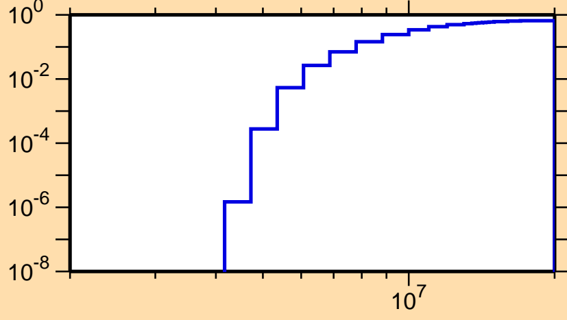
\sigma vs. E for ^{86}\text{Nb}(n,np)
