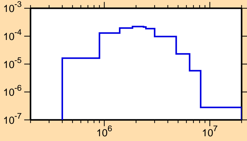
\sigma vs. E for ^{86}\text{Nb}(n,n_3)
