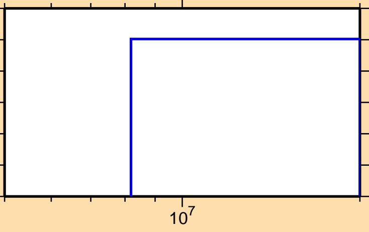
\sigma vs. E for ^{86}\text{Nb}(n,2np)
