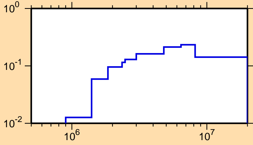
\sigma vs. E for ^{86}\text{Nb}(n,n\text{cont.})
