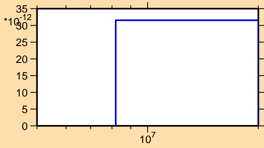
\sigma vs. E for ^{86}\text{Nb} (mt 34)
