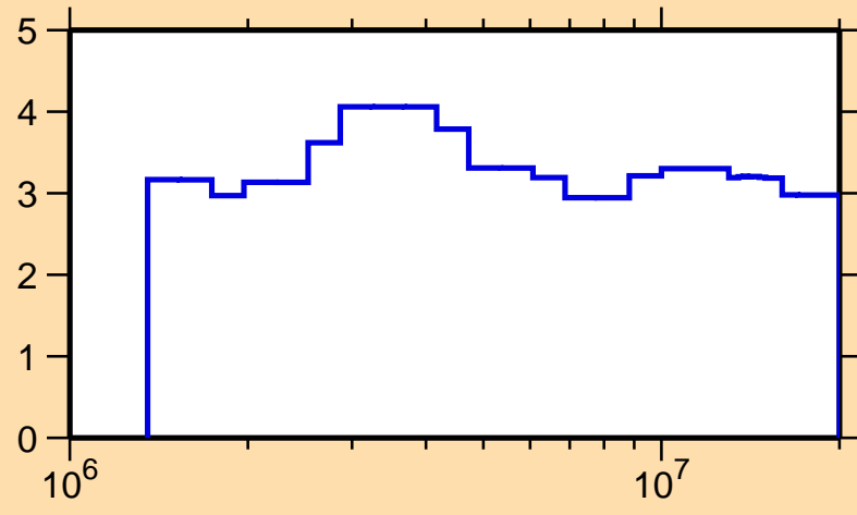
\Delta\sigma/\sigma vs. E for ^{87}\text{Nb}(n,n\text{nonel.})
