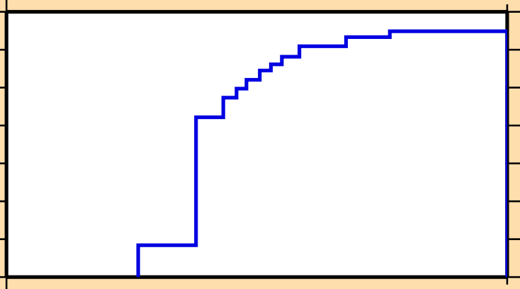
\sigma vs. E for ^{87}\text{Nb}(n,2n)
