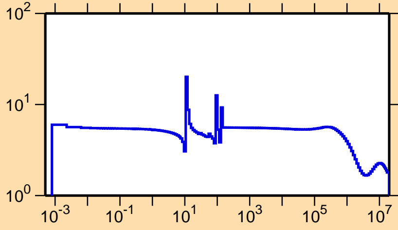
\sigma vs. E for ^{87}\text{Nb}(n,\text{el.})
