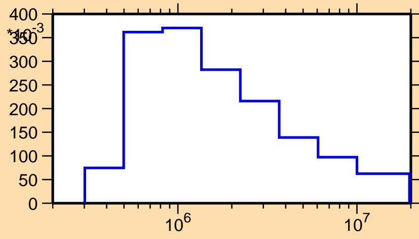
\sigma vs. E for ^{87}\text{Nb}(n,n_4)
