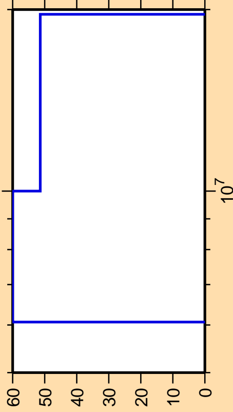
\Delta\sigma/\sigma vs. E for ^{87}\text{Nb}(n,n\alpha)
