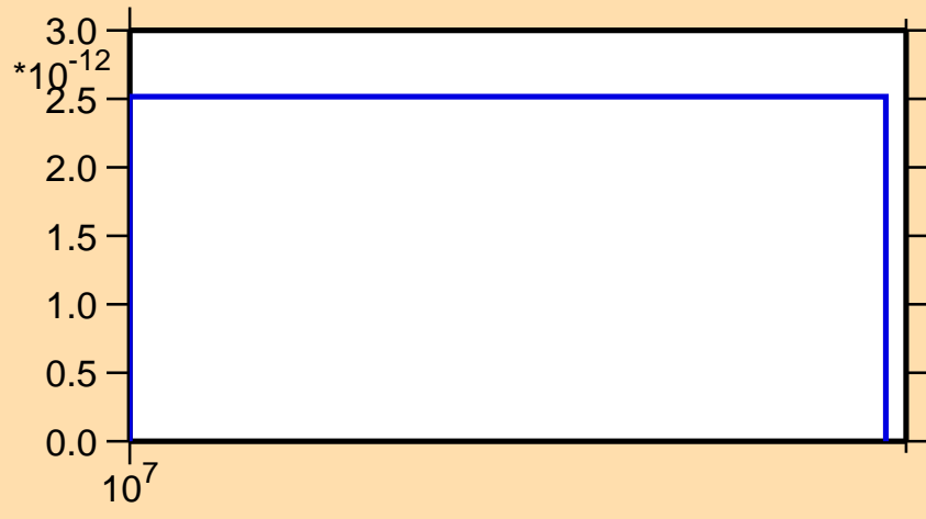
\sigma vs. E for ^{87}\text{Nb}(n,\text{pt})
