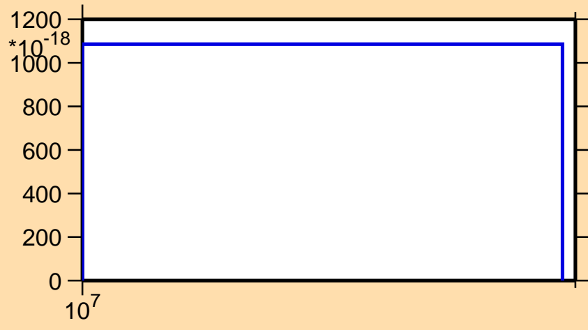
\sigma vs. E for ^{87}\text{Nb}(n,nt)
