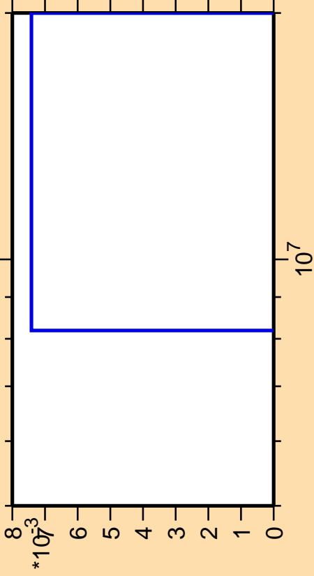
\Delta\sigma/\sigma vs. E for ^{87}\text{Nb} (mt 34)
