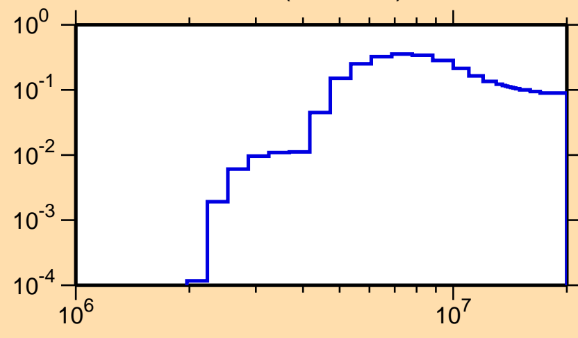
\sigma vs. E for ^{87}\text{Nb}(n,n\text{cont.})
