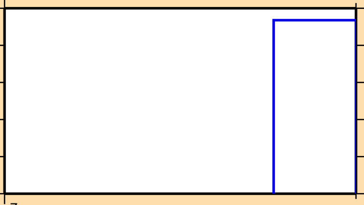
\sigma vs. E for ^{87}\text{Nb}(n,nt)
