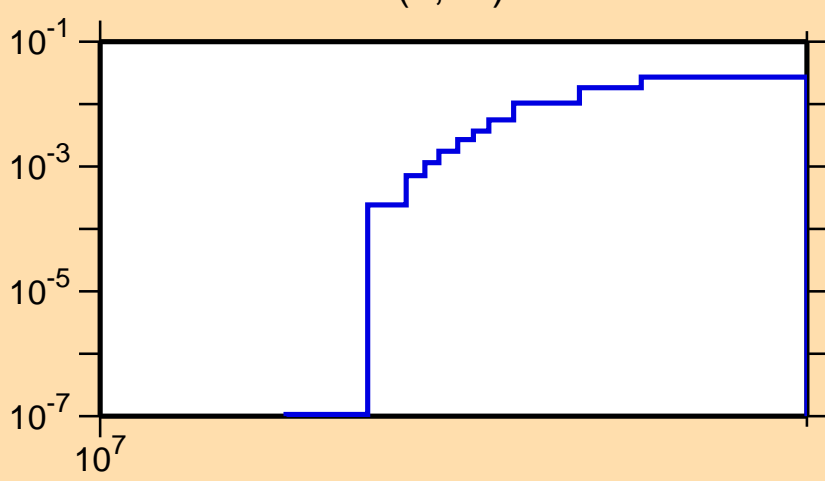
\sigma vs. E for ^{87}\text{Nb}(n,2n)
