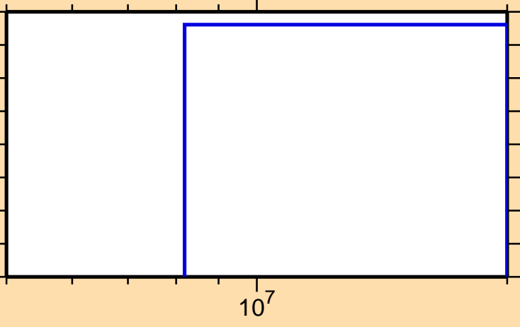
\sigma vs. E for ^{87}\text{Nb}(n,nt)
