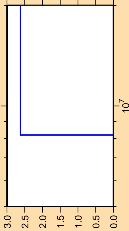
\Delta\sigma/\sigma vs. E for ^{87}\text{Nb}(n,\text{pt})
