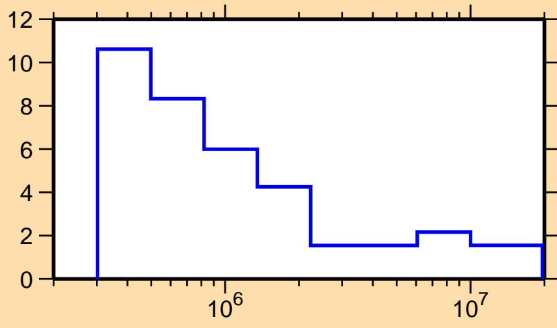
\Delta\sigma/\sigma vs. E for ^{88}\text{Nb}(n,n\text{onel.})
