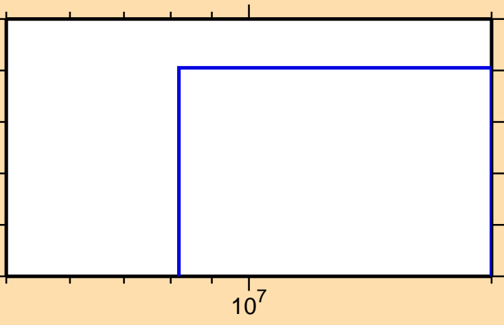
\sigma vs. E for ^{88}\text{Nb}(n,2n)
