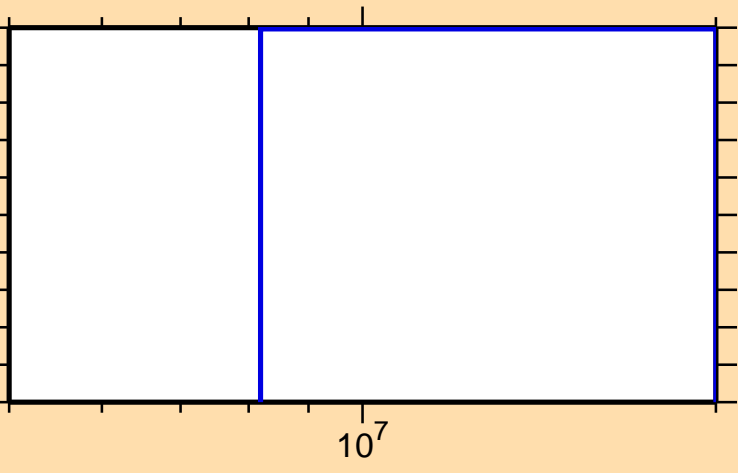
\sigma vs. E for ^{89}\text{Nb}(n,t)
