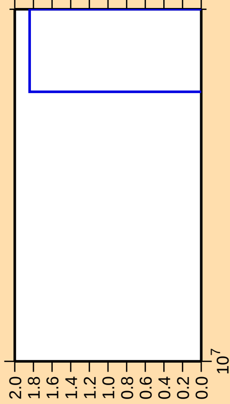
\Delta\sigma/\sigma vs. E for ^{89}\text{Nb}(n,\text{nt})
