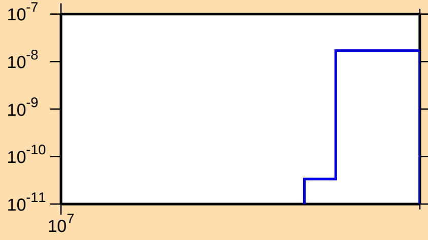
\sigma vs. E for ^{89}\text{Nb}(\text{mt } 45)
