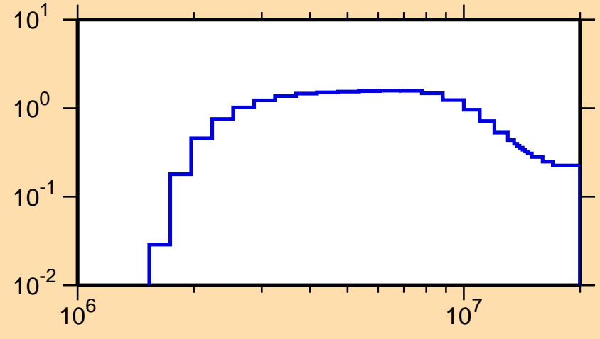
\sigma vs. E for ^{90}\text{Nb}(n,n\text{cont.})
