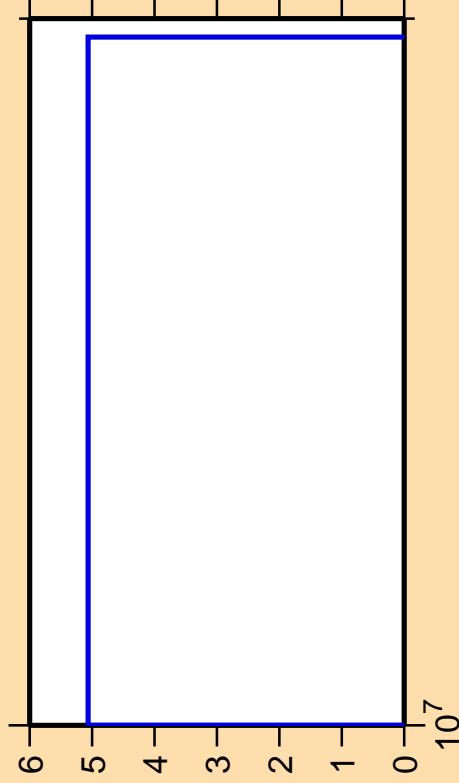
\Delta\sigma/\sigma vs. E for ^{90}\text{Nb}(n,\text{pt})
