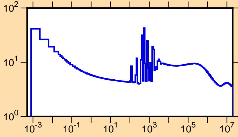
\sigma vs. E for ^{91}\text{Nb}(n,\text{tot.})
