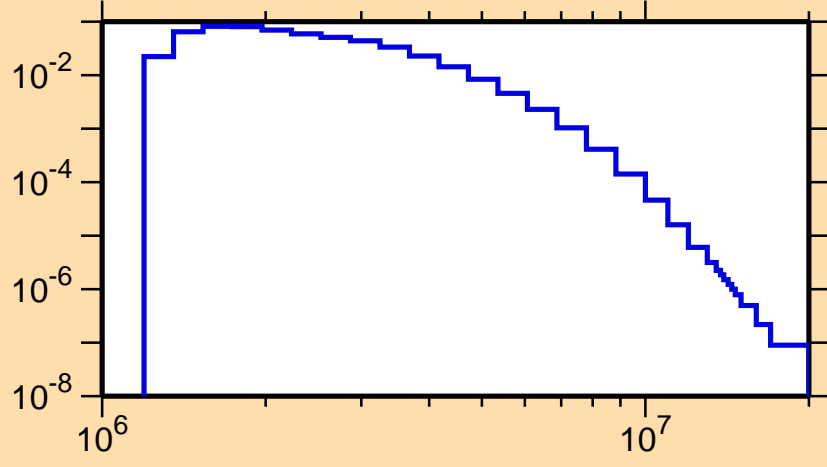
\sigma vs. E for ^{91}\text{Nb}(n,n_3)
