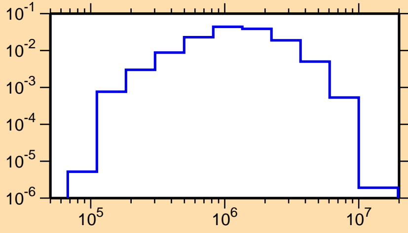
\sigma vs. E for ^{91}\text{Nb}(n,n_1)
