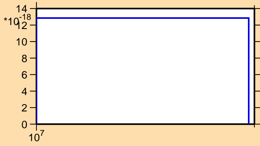
\sigma vs. E for ^{91}\text{Nb}(n,nt)
