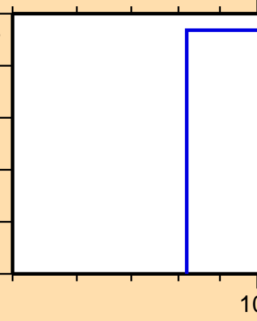
\sigma vs. E for ^{91}\text{Nb}(\text{mt117})
