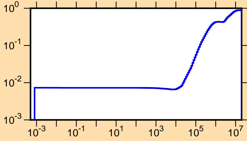
\mu vs. E for ^{92}\text{Nb}(\text{mt251})
