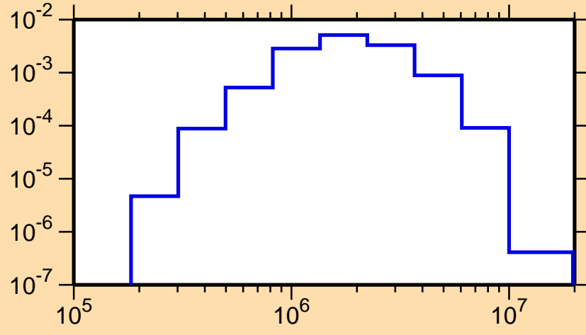
\sigma vs. E for ^{92}\text{Nb}(n,n_2)
