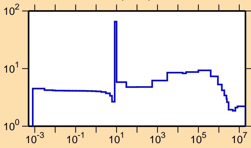
\sigma vs. E for ^{92}\text{Nb}(n,\text{el.})
