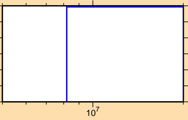
\sigma vs. E for ^{92}\text{Nb}(n,2np)
