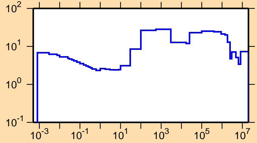
\Delta\sigma/\sigma vs. E for ^{92}\text{Nb}(n,\text{tot.})
