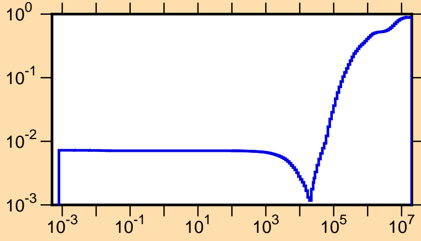
\mu vs. E for ^{93}\text{Nb}(\text{mt251})
