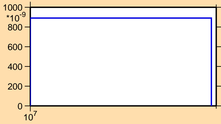
\sigma vs. E for ^{93}\text{Nb}(n,\text{nd})
