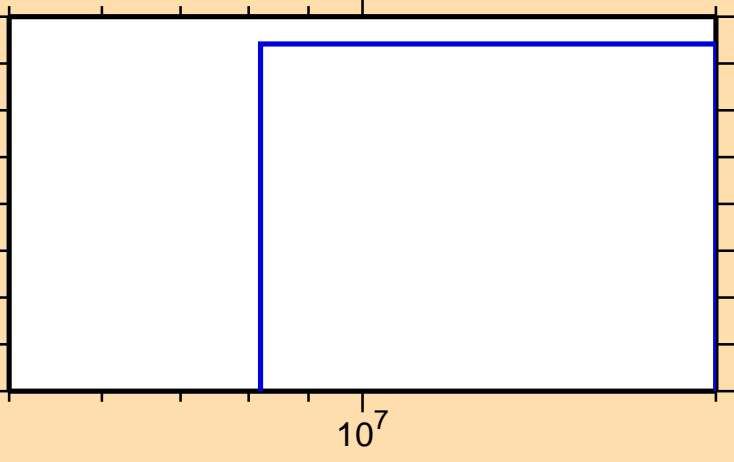
\sigma vs. E for ^{93}\text{Nb}(n,\text{nd})
