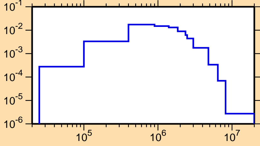
\sigma vs. E for ^{93}\text{Nb}(n,n_1)
