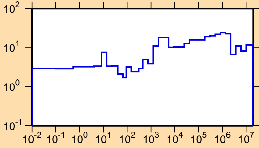
\Delta\sigma/\sigma vs. E for ^{94}\text{Nb}(n,el.)
