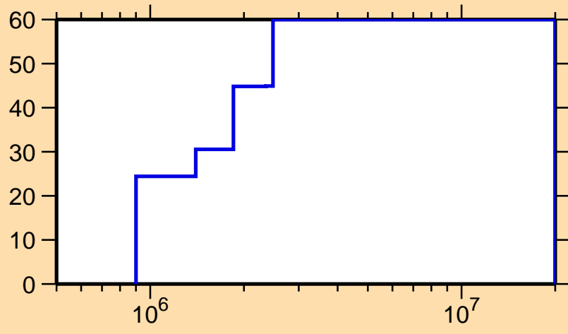
\Delta\sigma/\sigma vs. E for ^{94}\text{Nb}(n,n_1)
