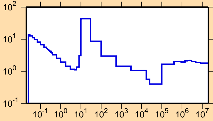
\sigma vs. E for ^{94}\text{Nb}(n,\text{nonel.})
