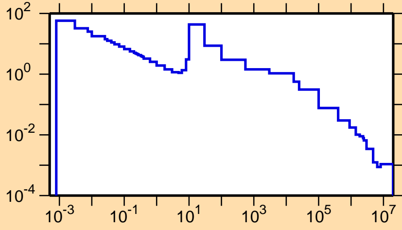
\sigma vs. E for ^{94}\text{Nb}(n,\gamma)
