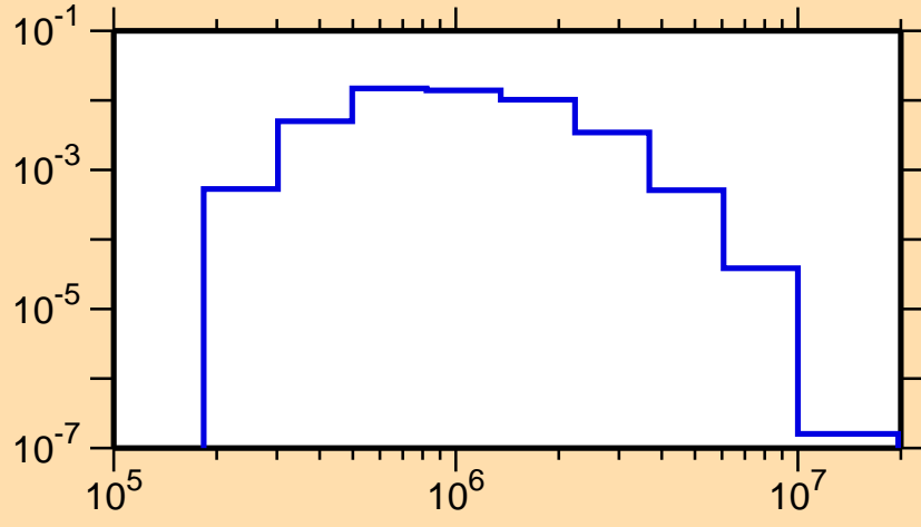
\sigma vs. E for ^{95}\text{Nb}(n,n_1)
