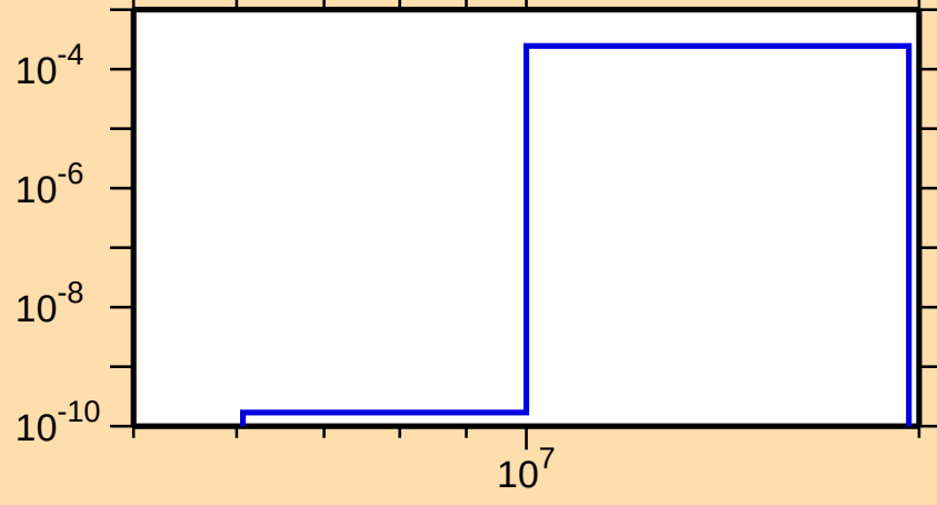
\sigma vs. E for ^{95}\text{Nb}(n,t)
