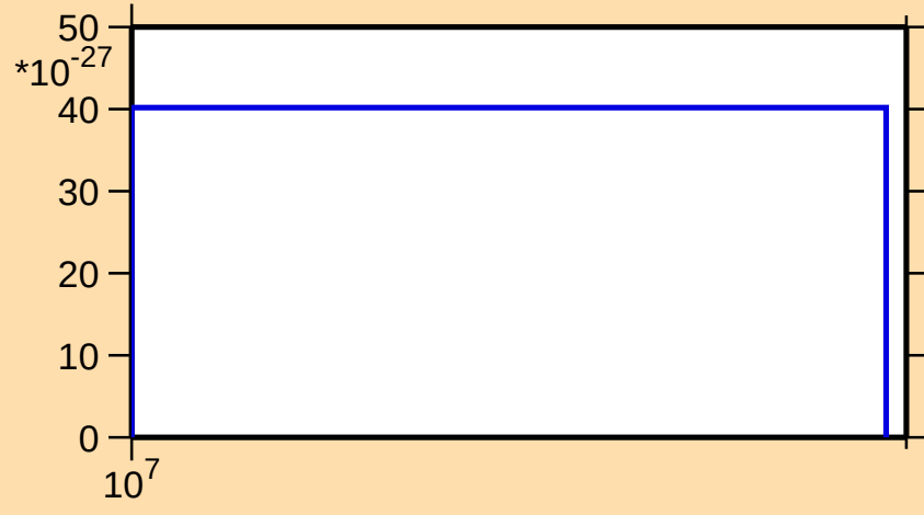
\sigma vs. E for ^{95}\text{Nb}(\text{mt } 11)
