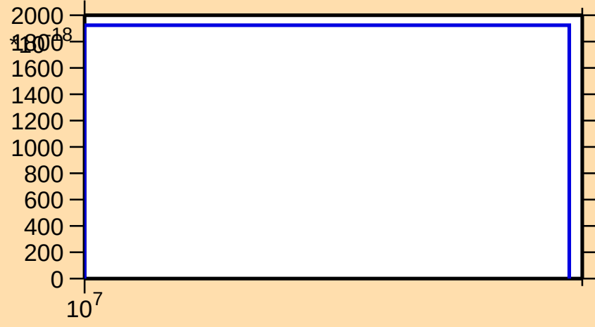
\sigma vs. E for ^{95}\text{Nb}(\text{mt } 45)
