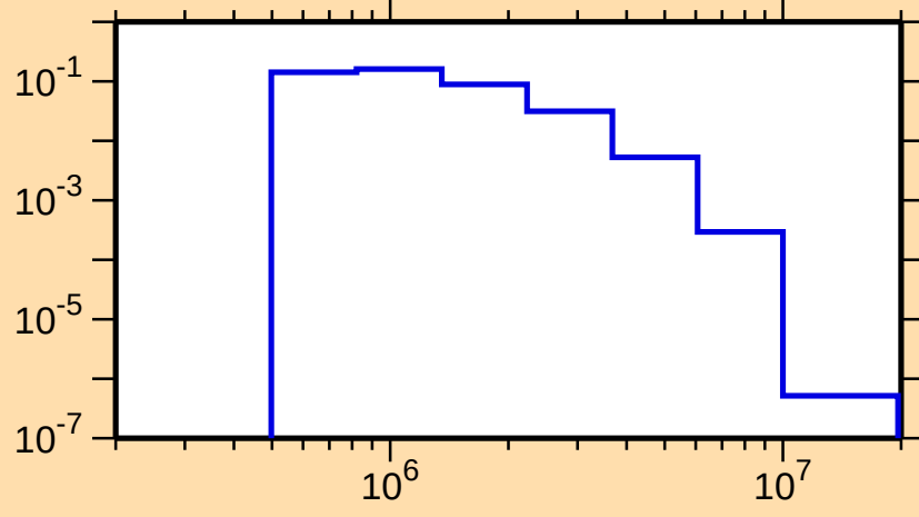
\sigma vs. E for ^{95}\text{Nb}(n,n_3)
