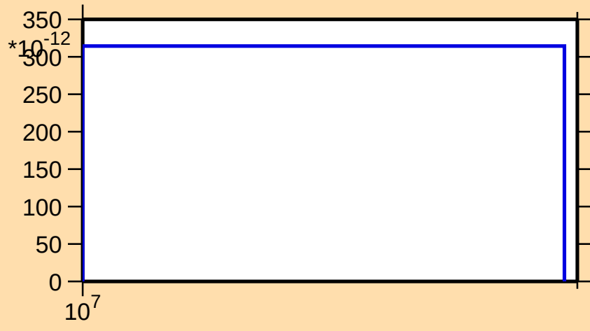
\sigma vs. E for ^{95}\text{Nb}(n,p\alpha)
