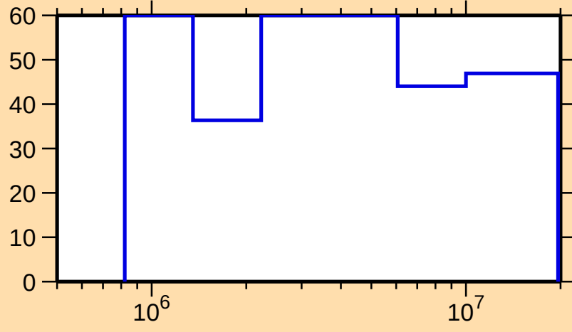
\Delta\sigma/\sigma vs. E for ^{95}\text{Nb}(n,p)
