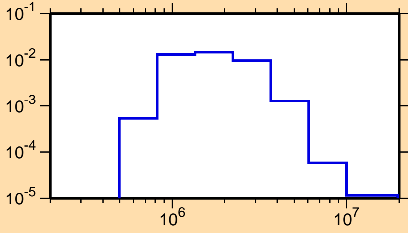
\sigma vs. E for ^{97}\text{Nb}(n,n_1)
