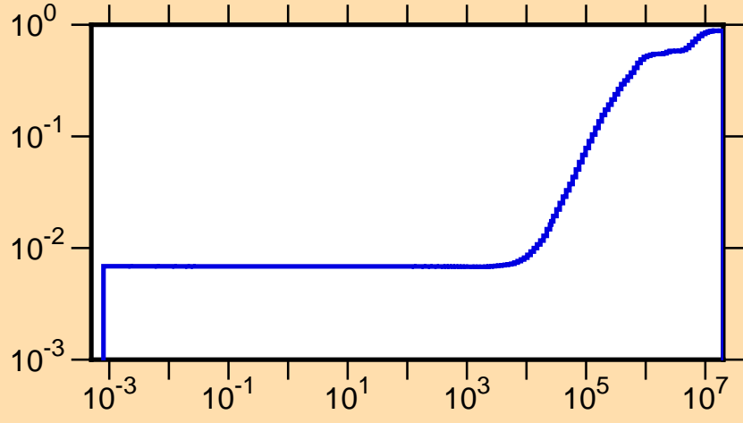
\mu vs. E for ^{98}\text{Nb}(\text{mt251})
