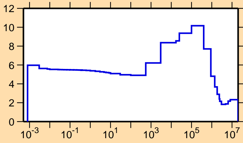
\sigma vs. E for ^{98}\text{Nb}(n,\text{el.})
