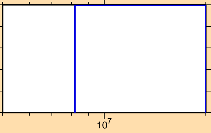
\sigma vs. E for ^{99}\text{Nb}(n,2np)
