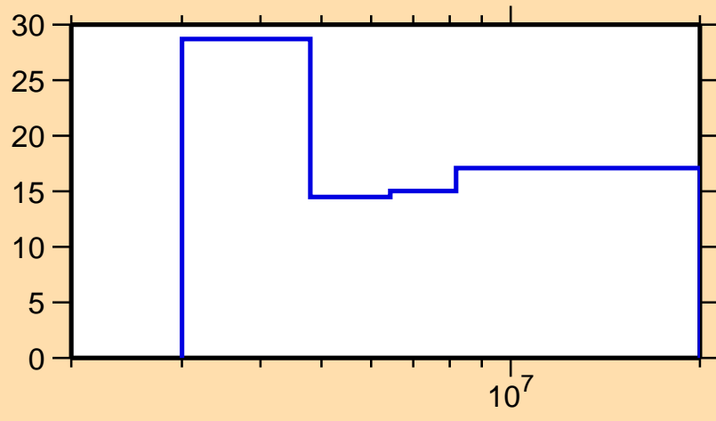
\Delta\sigma/\sigma vs. E for ^{99}\text{Nb}(n,el.)
