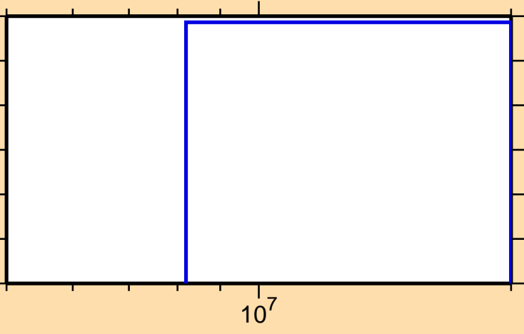
\sigma vs. E for ^{99}\text{Nb}(n,np)
